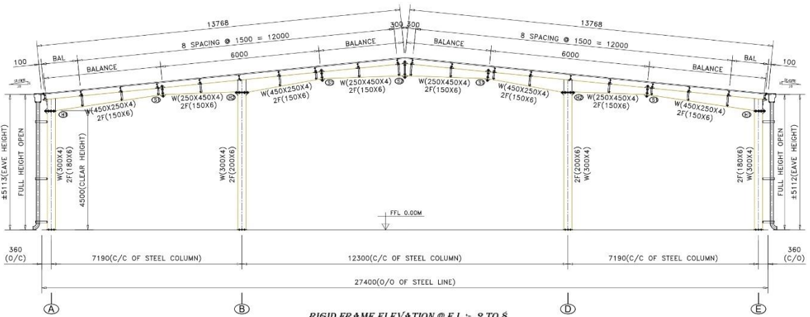
RIGID FRAME ELEVATION @ F.L.:- 2 TO 8 ↑↑ DOUBLE SIDED FLANGE BRACE
