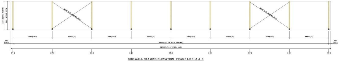
SIDEWALL FRAMING ELEVATION : FRAME LINE A & E
